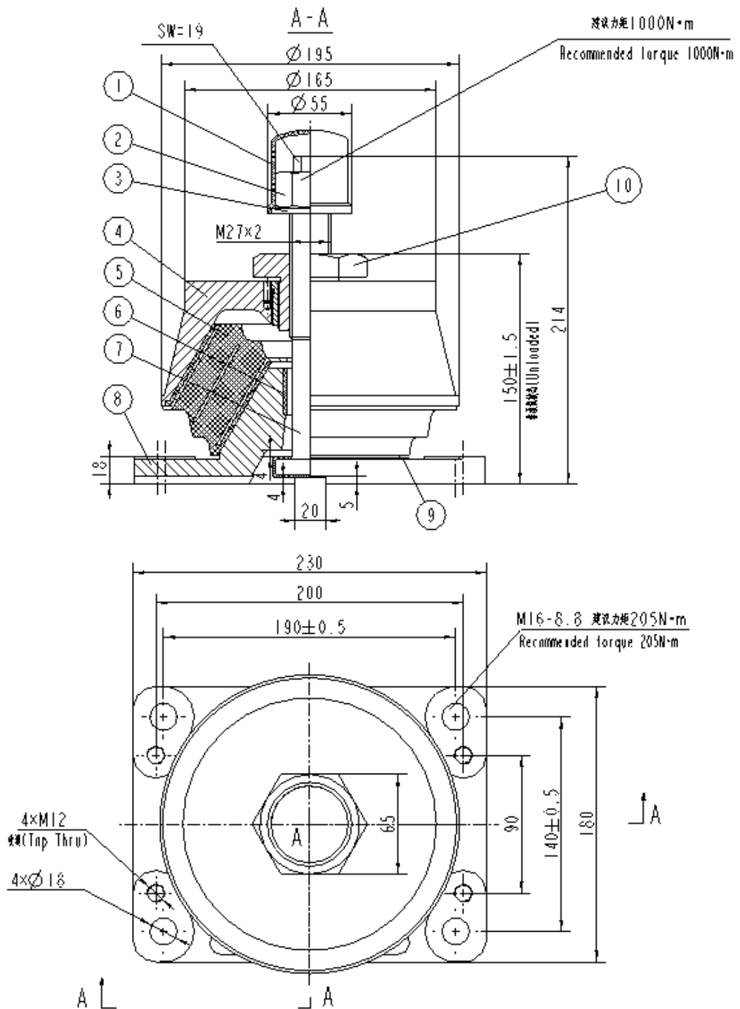
Fig (1) CM-IV type vibration isolator
