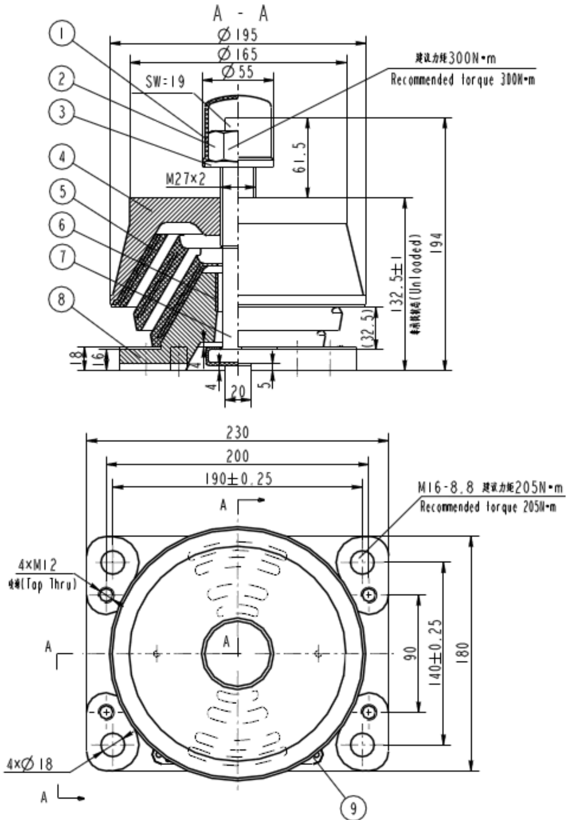
Fig (1) CM-V-1 type vibration isolator
