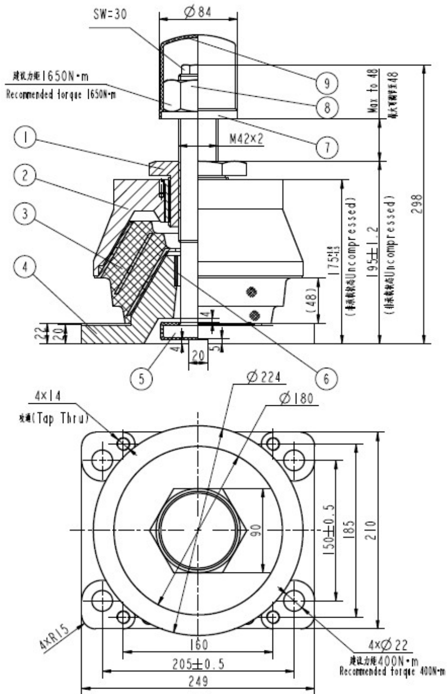
Fig (1) CM-VII type vibration isolator
